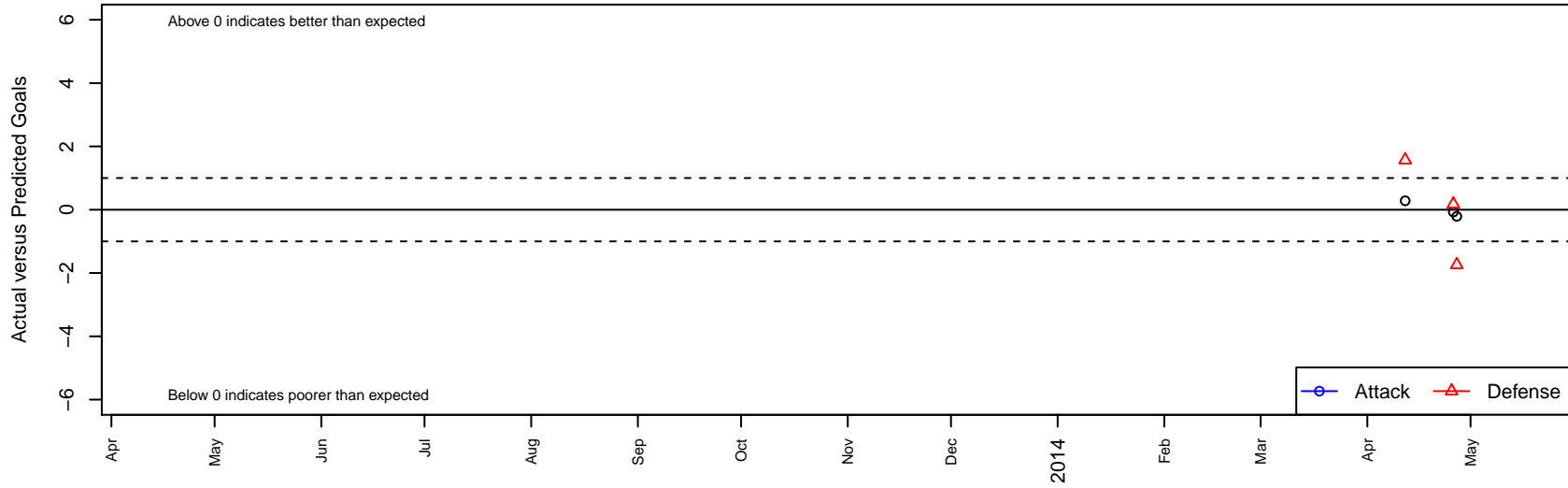
Santa Barbara SC White B99 Dots are actual minus expected GF (blue circles) and GA (red triangles). Blue line is smoothed change in attack strength. Red is smoothed change in defense strength.
